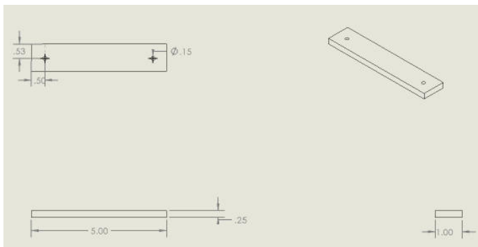
Chassis link
