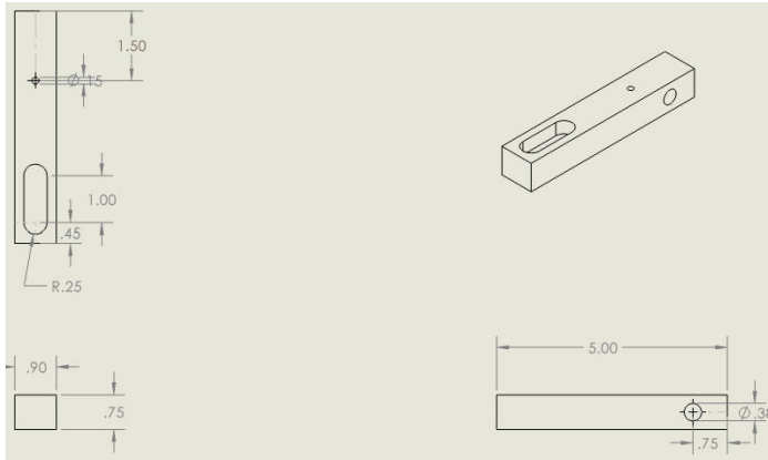
Wheel link dimensions
