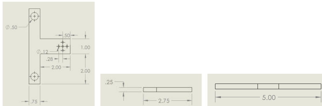
Servo link's dimensions top, front and right sides respectively.
