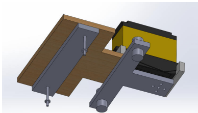
Straight link screwed into chassis.
